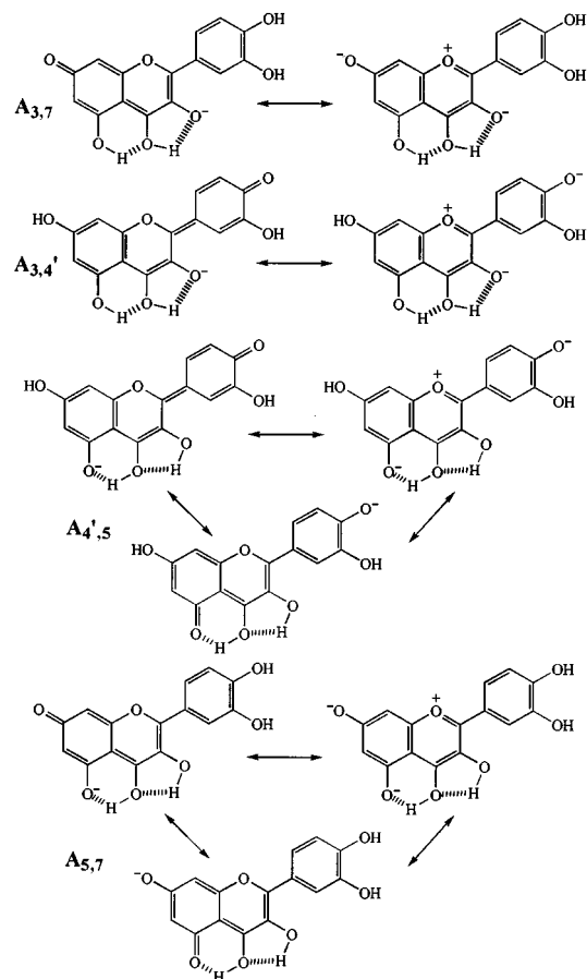
Scheme 2
