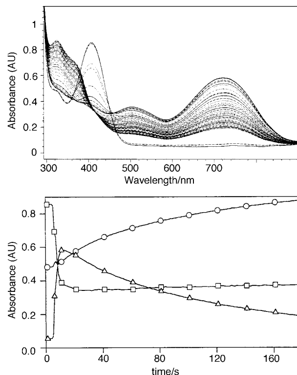
Fig. 5 Upper part: changes in the UV-visible spectrum of quercetin ( 5 \times 10^{-5} \text{ mol dm}^{-3} ) after addition of sodium periodate (1 equiv) in a pH 9.0 buffer containing BSA ( 7.52 \times 10^{-5} \text{ mol dm}^{-3} ) (25 °C, ionic strength: 0.2 \text{ mol dm}^{-3} ). Lower part: kinetic traces at 723 ( \Delta ), 406 ( \square ) and 324 nm ( \circ ).
