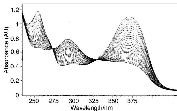
Fig. 3 Changes in the UV–visible spectrum of quercetin ( 5 \times 10^{-5} mol \text{dm}^{-3} ) after addition of sodium periodate (1 equiv) in methanol at 25 °C. Time interval: 0–2 h.
