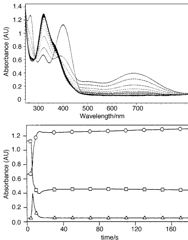
Fig. 4 Upper part: changes in the UV-visible spectrum of quercetin ( 5 \times 10^{-5} \text{ mol dm}^{-3} ) after addition of sodium periodate (1 equiv) in a pH 9.0 buffer (25 °C, ionic strength: 0.2 \text{ mol dm}^{-3} ). Lower part: kinetic traces at 690 ( \Delta ), 402 ( \square ) and 324 nm ( \circ ).
