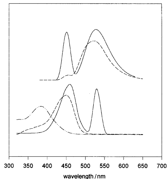
Fig. 2 Upper part: emission spectra of quercetin bound to BSA (solid line, quercetin–BSA molar ratio = 2, pH 7.4 phosphate buffer) and in HBr (1 mol dm -3 )–acetic acid (broken line). Excitation wavelength: 450 nm. Lower part: excitation spectrum of BSA-bound quercetin (solid line, emission wavelength: 530 nm, quercetin–BSA molar ratio = 2, pH 7.4 phosphate buffer), absorption spectra of quercetin bound to BSA (dotted line, quercetin–BSA molar ratio = 2, pH 7.4 phosphate buffer) and in HBr (1 mol dm -3 )–acetic acid (broken line).
