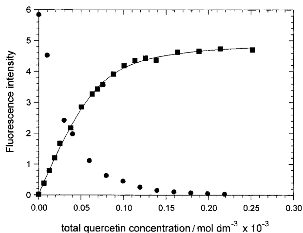
Fig. 1 Plot of the fluorescence intensity as a function of the total quercetin concentration in a pH 7.4 buffer containing BSA ( 7.52 \times 10^{-5} mol dm ^{-3} ) (25 °C, ionic strength: 0.2 mol dm ^{-3} ). Squares: emission at 530 nm (excitation wavelength: 450 nm). The solid line is the result of the curve-fitting procedure (Scatchard analysis). Circles: emission at 340 nm (excitation wavelength: 295 nm).
